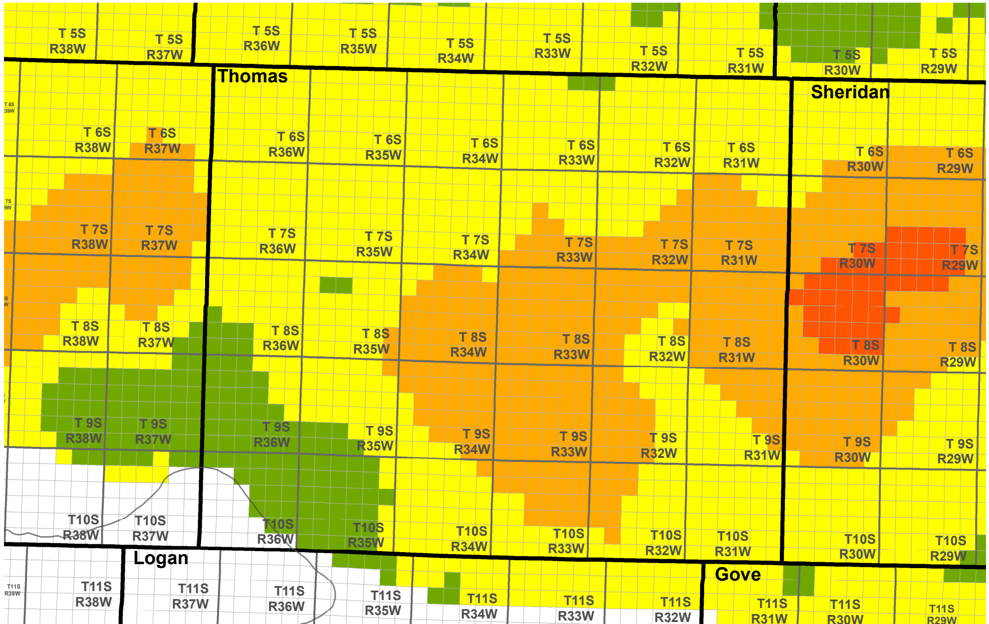
Rate of groundwater decline (Feet per year)
