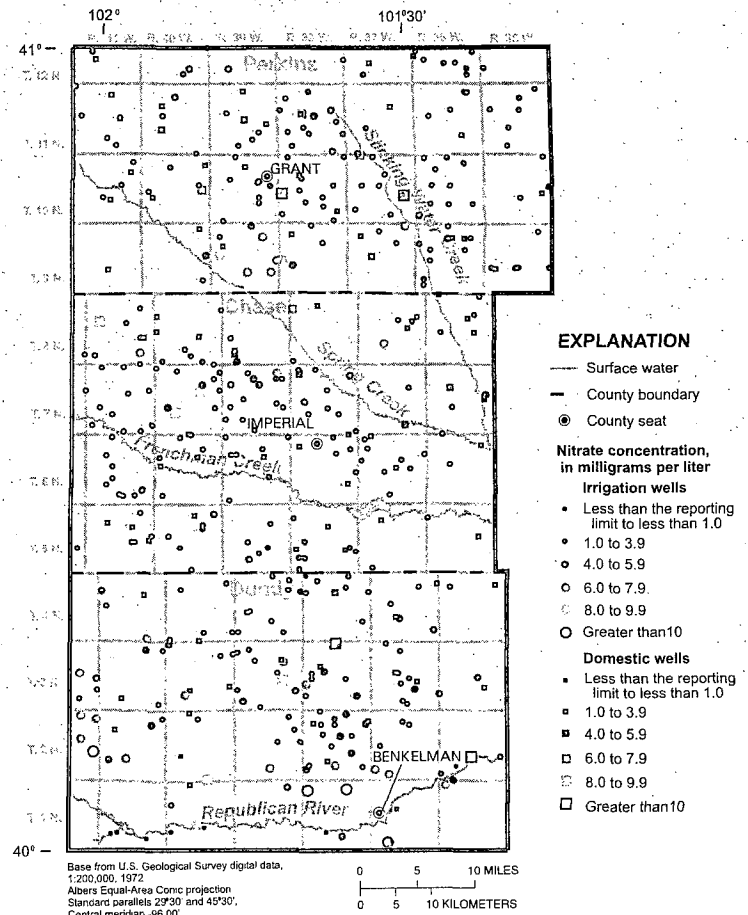
Figure 3. Approximate locations and concentrations of nitrates detected in water from irrigation and domestic wells sampled in the Upper Republican Natural Resources District, Nebraska, June–August 1998.
