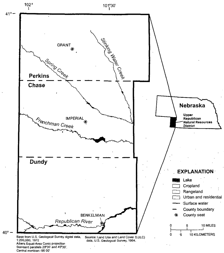
Figure 1. Location of and land uses in the Upper Republican Natural Resources District, southwestern Nebraska.
