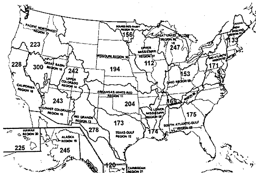
Average use per person (gall/day) of public water in the United States by USGS water region (Solley et al., 1993)
