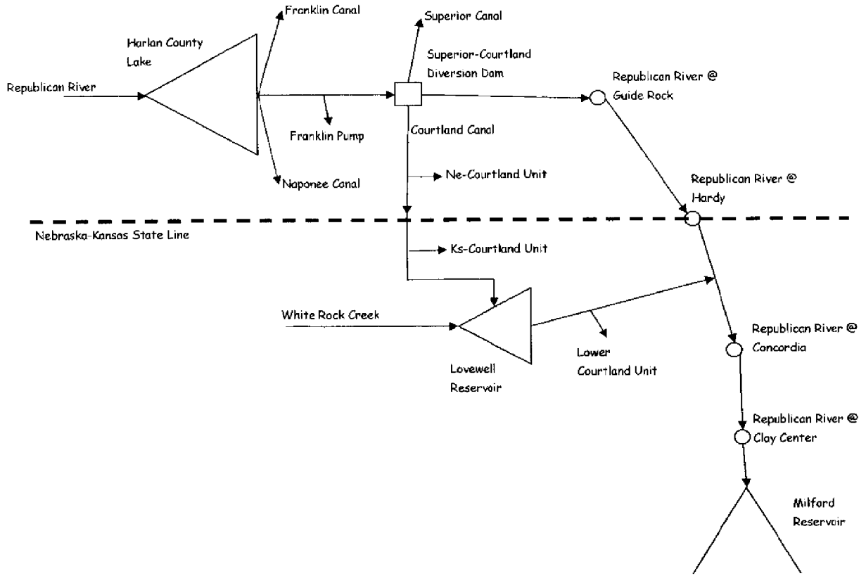
Figure 1 - Schematic Diagram of Lower Republican River Basin
