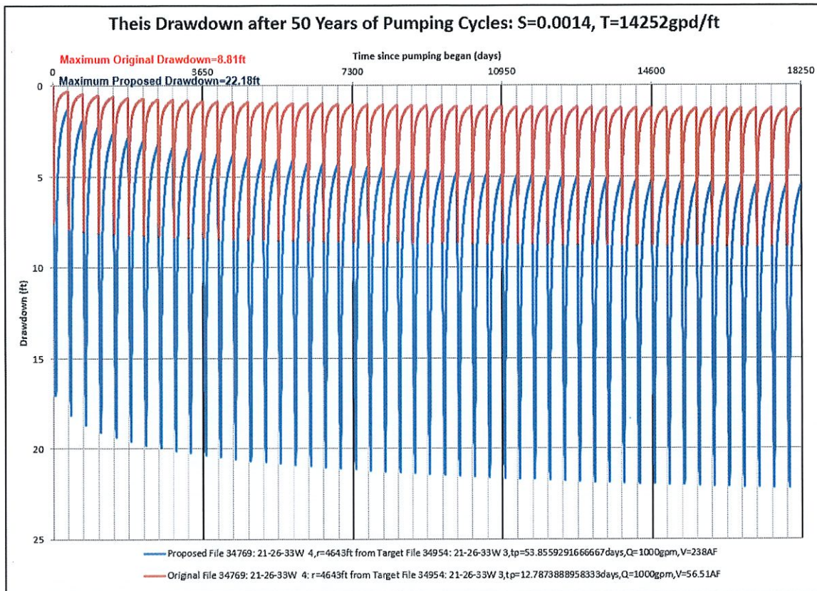
Figure 3: This drawdown of pumping 238 AF from well 34,769 at target well 34,954
