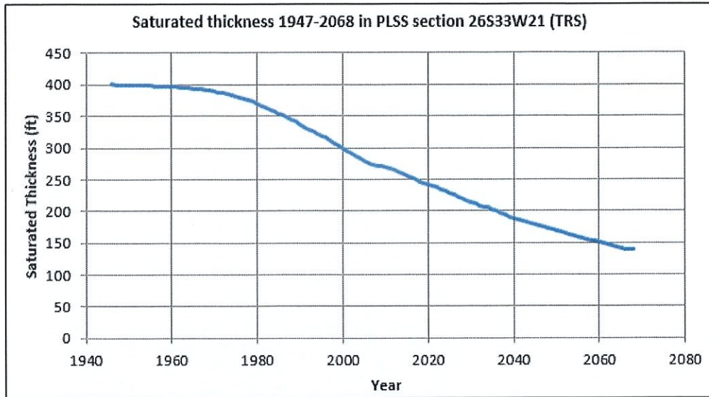
Figure 1 Projected saturated thickness (GMD No. 3 groundwater model)
