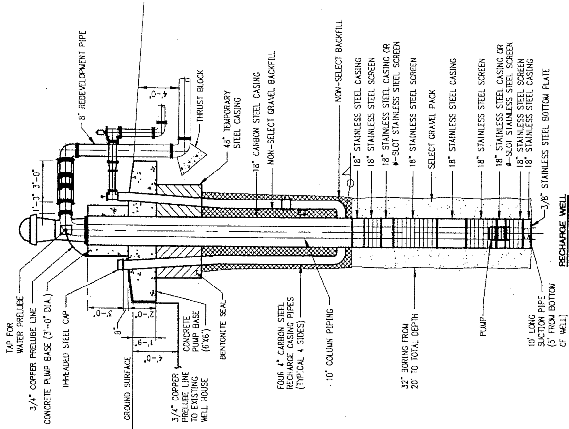
Figure 10. – Application No. 45568 Example of Construction Design for Recharge and Recovery Well
