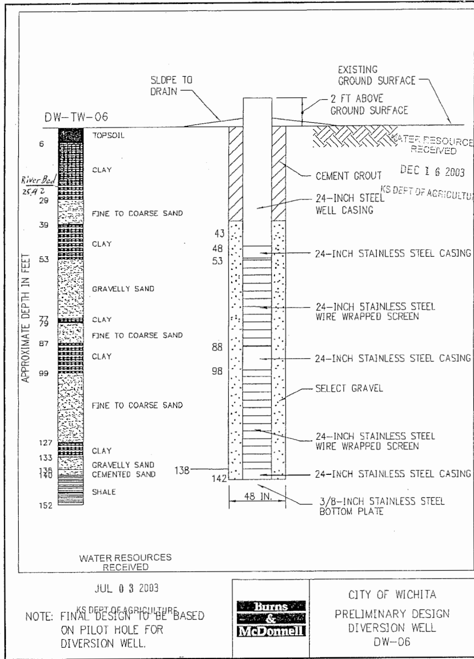
Figure 4. – Application No. 45570 Lithologic Log and Construction Design for Bank Storage Well
