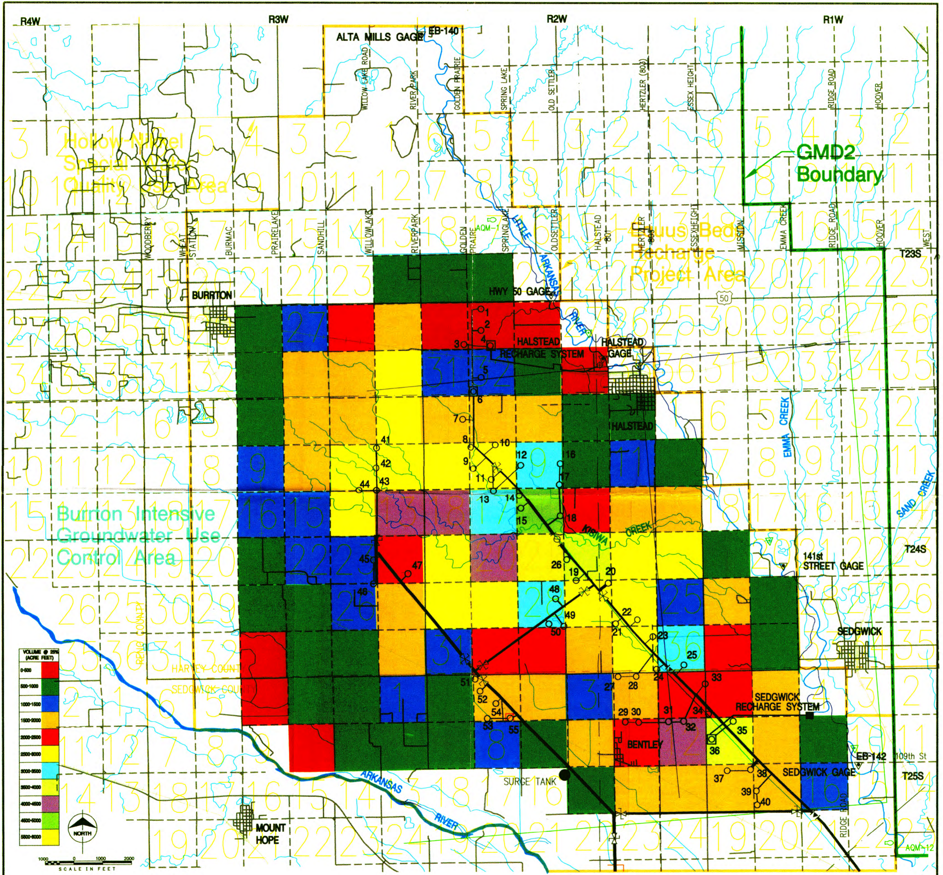
Figure VII-25 15 AVAILABLE AQUIFER STORAGE VOLUME BY SECTION
