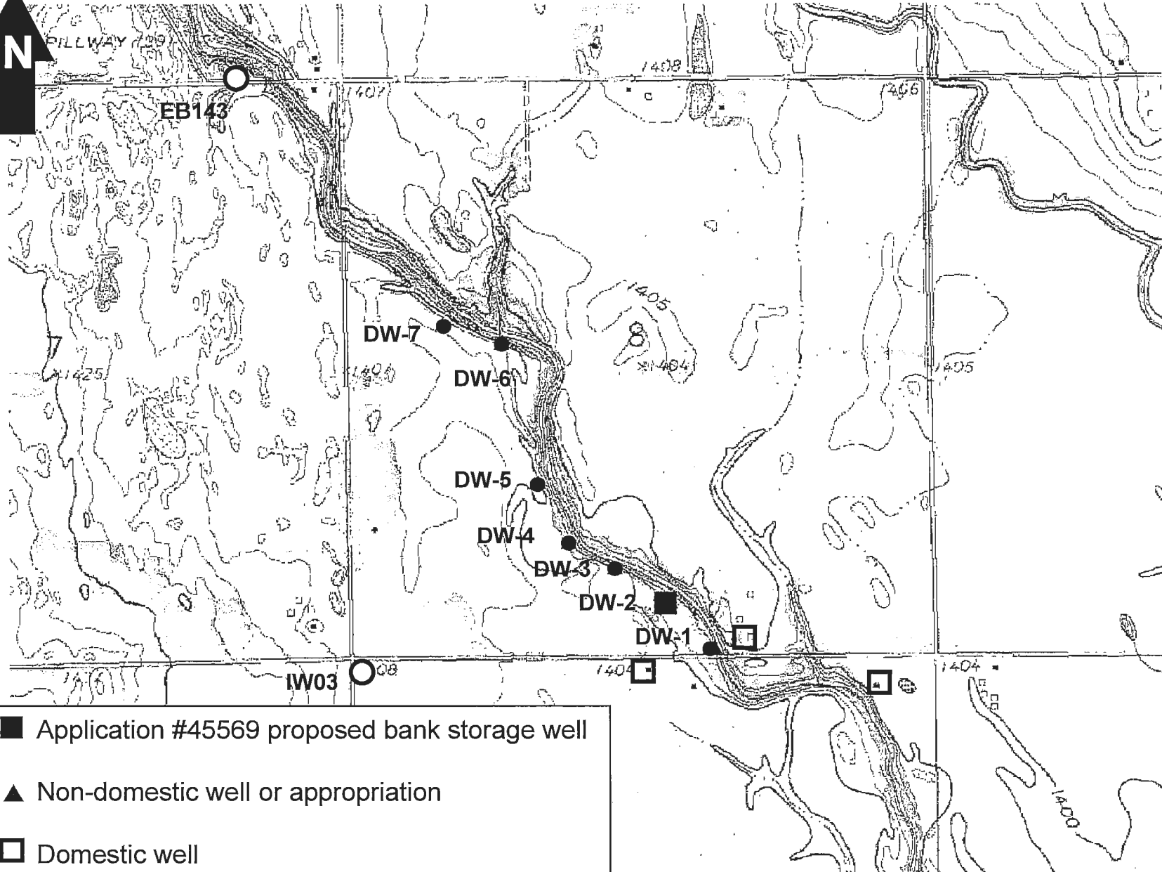
Figure 3. – Application No. 45569 Site Map - SE 08-23S-2W Prepared by: Equus Beds Groundwater Management District No. 2 - 07/06/04
