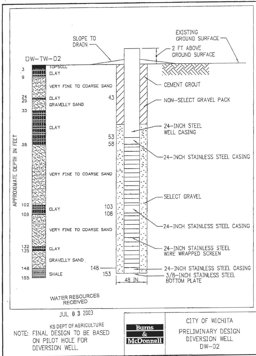
Figure 4. – Application No. 45569 Lithologic Log and Construction Design for Bank Storage Well
