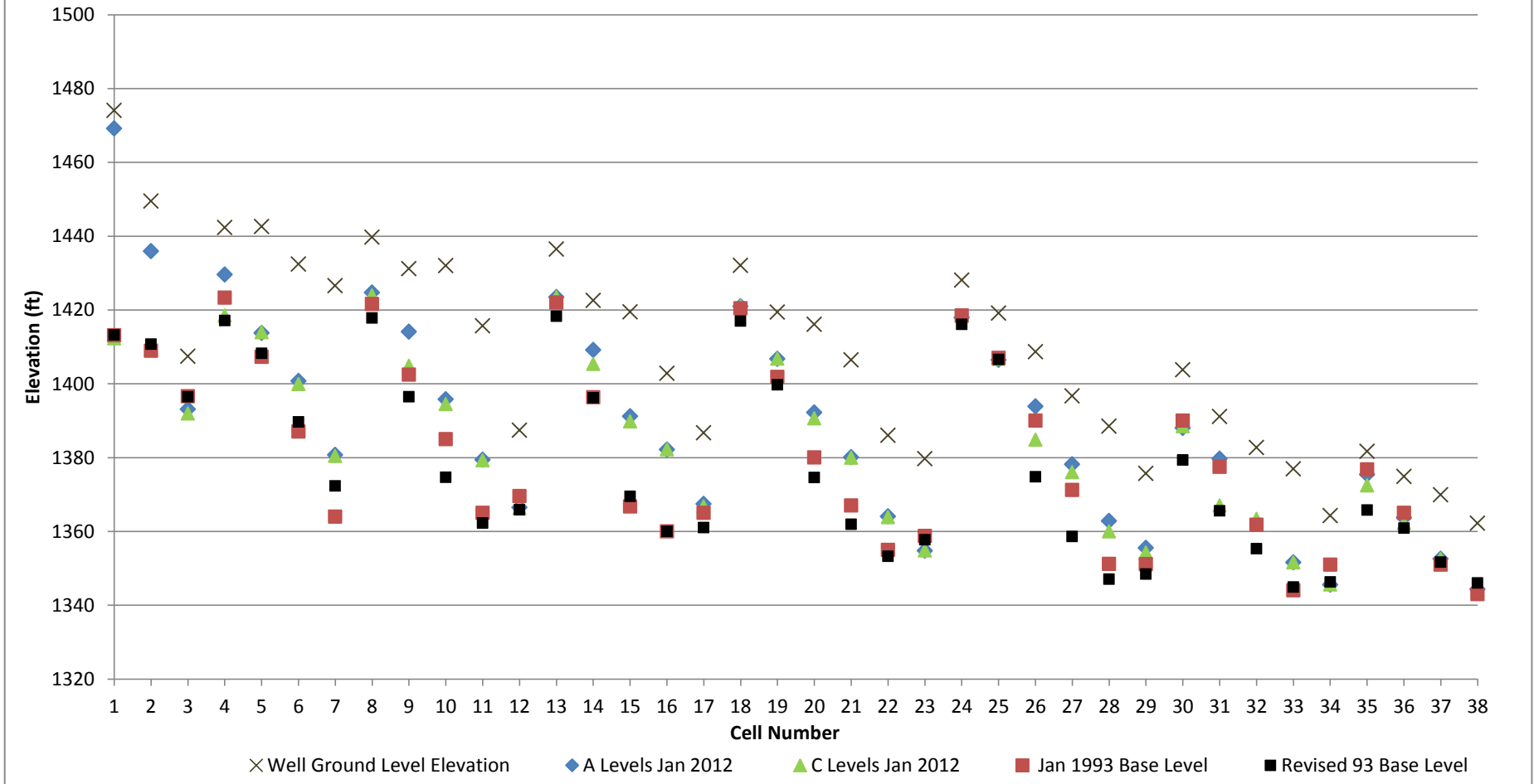
Wichita ASR Comparison of Jan 2012 A & C Groundwater Levels to 1993 Base Levels
